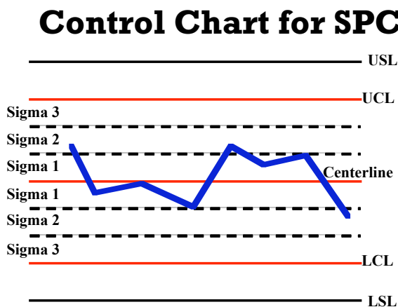
Figure 3. The upper and lower control limits of an effective SPC program are comfortably within the upper and lower specification limits.
