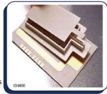
Figure 2-1 Foster-Miller LCP based RF circuit board and hermetic enclosure shapes (courtesy of Foster-Miller and Quantum Leap Packaging)
