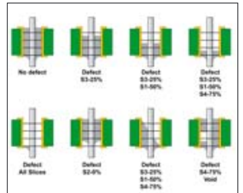
Figure 4: Data reporting scenarios for through-hole penetration based on 5DX analysis
