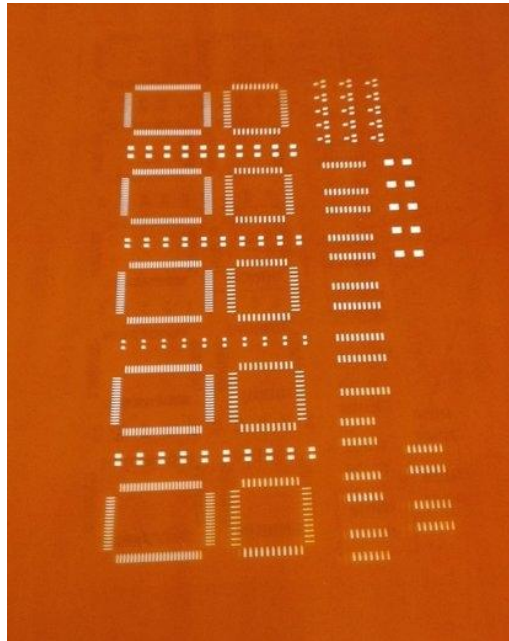
Figure 4 Kapton(TM) Stencil
