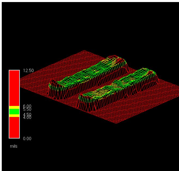
Figure 13-U6, Location 1 Showing "scooping" effect of Kapton™
