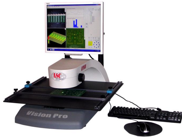
Figure 6-ASC Vision Pro 5000 used for SPI measurements
