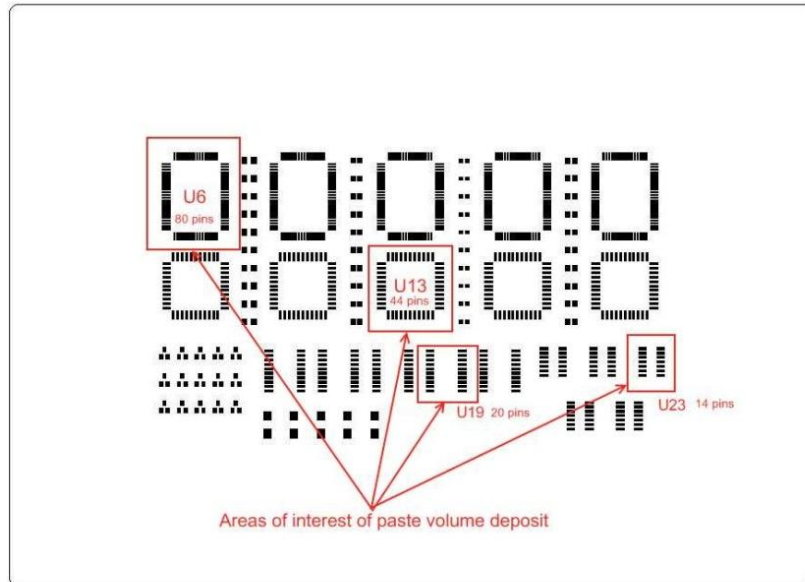
Figure 3-Location designators where solder paste volume measured with SPI
