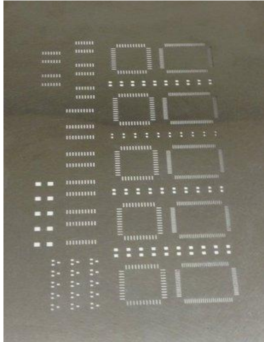
Figure 5-PHD stainless steel stencil
