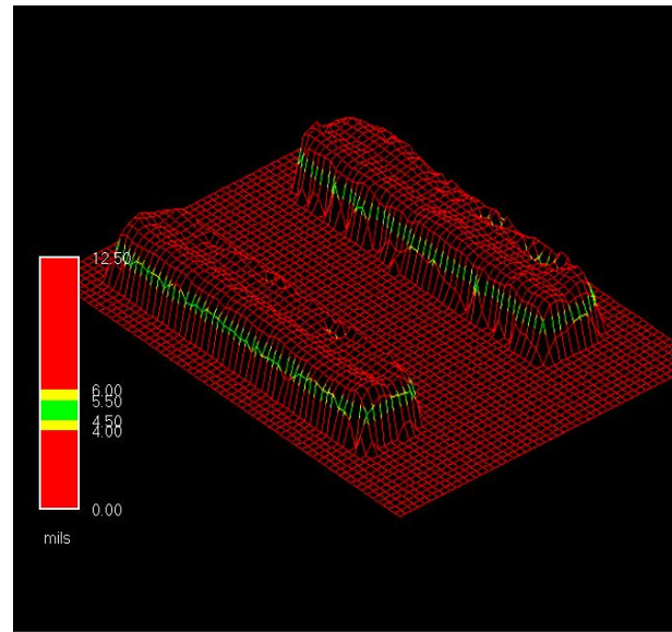
Figure 16- Stainless stencil U19, Location 3
