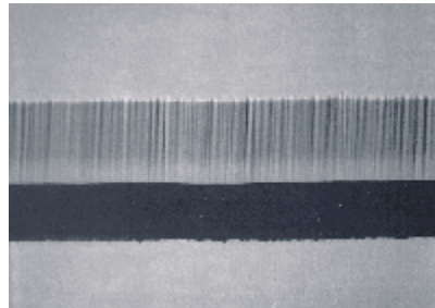
Figure 2-Typical stainless steel side wall
