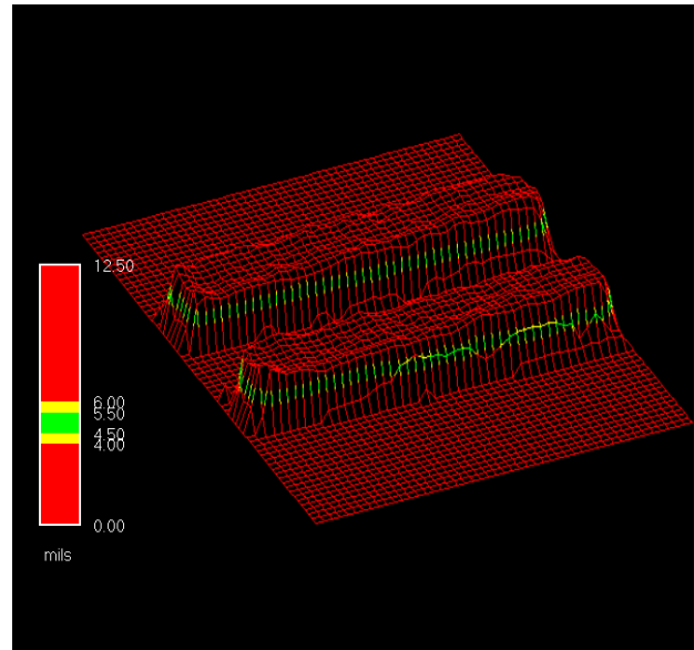
Figure 14- U6, Location 1 Stainless stencil
