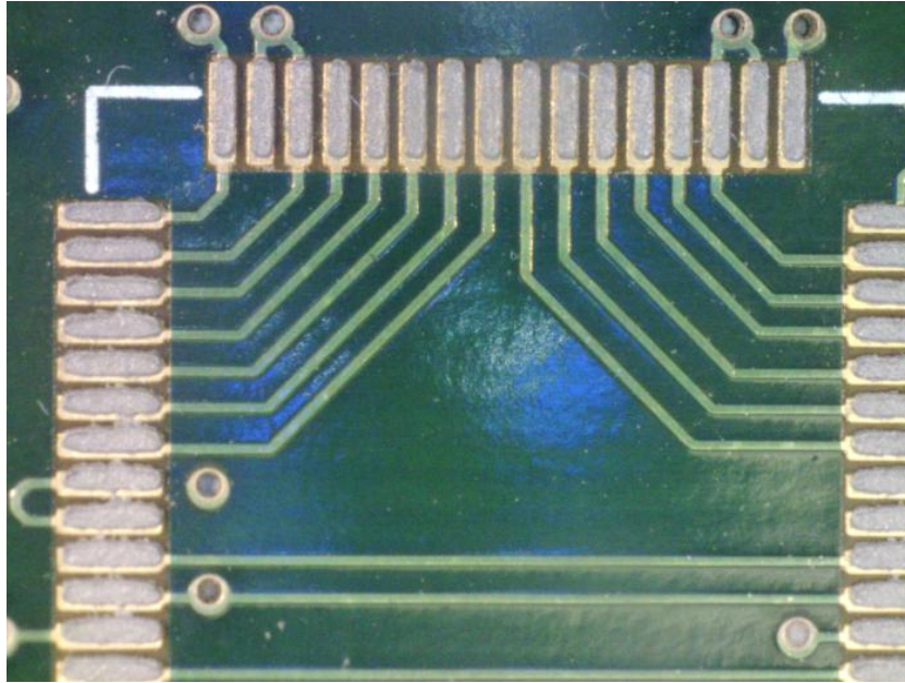
Figure 12-Kapton(TM) stencil print example showing smeared paste at U6
