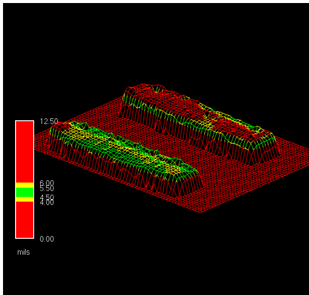
Figure 15-Kapton(TM) stencil "scooping" effect at U19, Location 3
