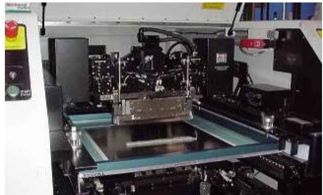
Figure 9. MPM Stencil Printer
