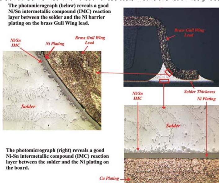
Figure 9. Cross-sectional tests for SMD parts
