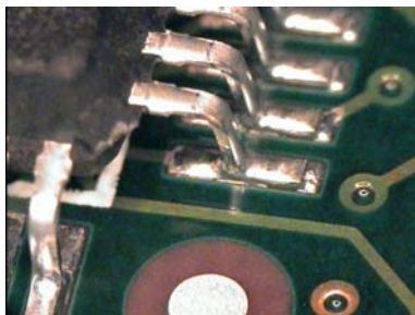
Figure 8. Various SMD parts soldered well with SAC305; all met IPC-610 Class 1, 2, 3
