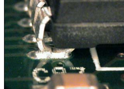
Figure 8. Various SMD parts soldered well with SAC305; all met IPC-610 Class 1, 2, 3
