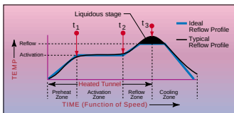
Figure 1. An example of a theoretically ideal reflow profile made up of four parts or zones - the first three are heating and the last is cooling.
