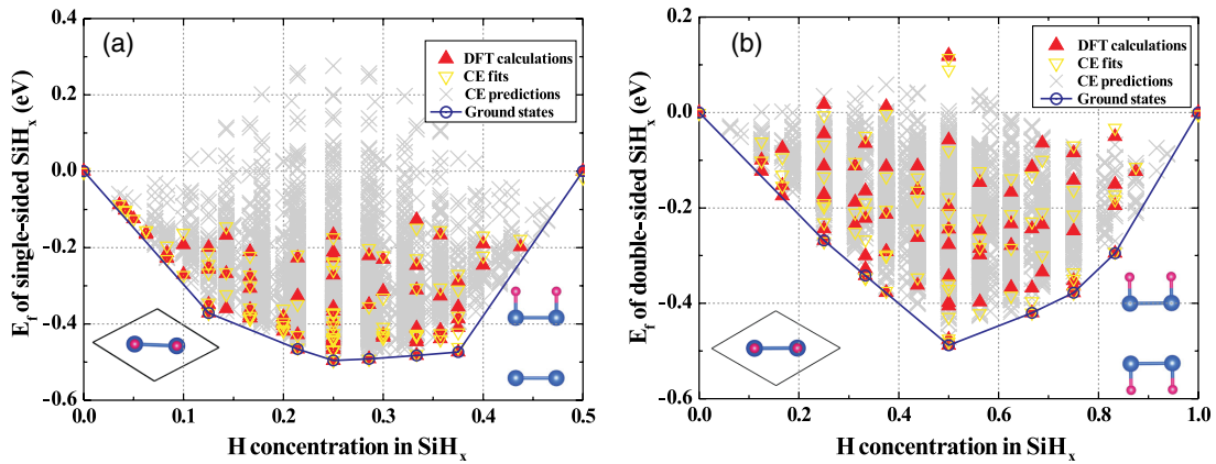
FIG. 2. (a) The calculated formation energies E_f of single-sided \text{SiH}_x along with the corresponding CE fits as a function of x . The E_f of all the symmetry-inequivalent structures calculated from CE are also plotted here. Inset: The top and side views of the structures of \text{SiH}_{0.5} . Panel (b) is the same as (a) but for double-sided \text{SiH}_x . The top and side views of the \text{SiH}_1 structure are also shown in Fig. 2(b).
