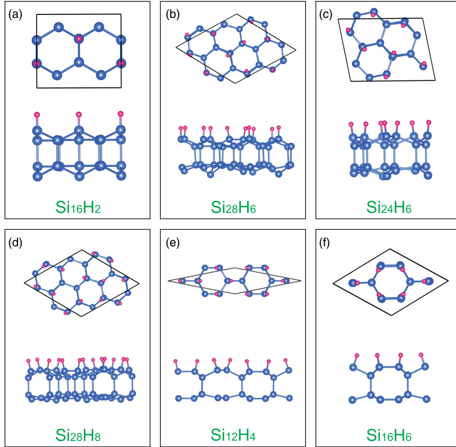
FIG. 3. The top and side views of six CE-discovered intermediate ground-state structures for single-sided (a) \text{Si}_{16}\text{H}_2 , (b) \text{Si}_{28}\text{H}_6 , (c) \text{Si}_{24}\text{H}_6 , (d) \text{Si}_{28}\text{H}_8 , (e) \text{Si}_{12}\text{H}_4 , and (f) \text{Si}_{16}\text{H}_6 .
