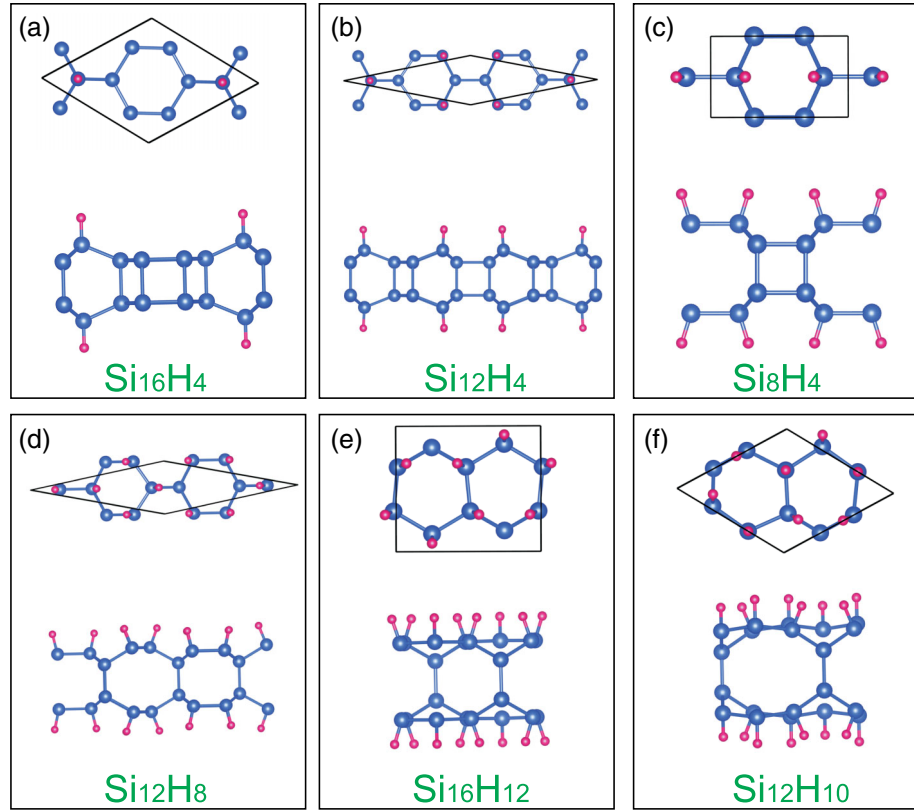
FIG. 4. The top and side views of six CE-discovered intermediate ground-state structures for double-sided (a) \text{Si}_{16}\text{H}_4 , (b) \text{Si}_{12}\text{H}_4 , (c) \text{Si}_8\text{H}_4 , (d) \text{Si}_{12}\text{H}_8 , (e) \text{Si}_{16}\text{H}_{12} , and (f) \text{Si}_{12}\text{H}_{10} .
