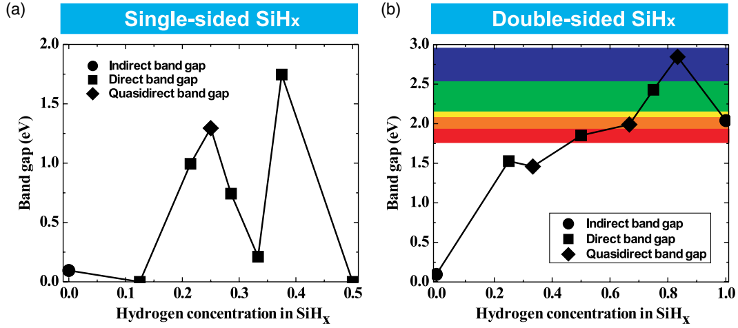
FIG. 5. The calculated band gaps of (a) single-sided \text{SiH}_x and (b) double-sided \text{SiH}_x ground states as a function of hydrogen concentration. In panel (b), a sketch of light spectrum is overlaid to aid visualization of the size of band gap.
