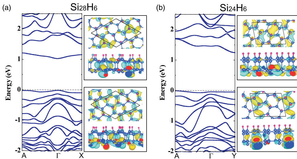
FIG. 6. The calculated band structures of single-sided (a) \text{Si}_{28}\text{H}_6 and (b) \text{Si}_{24}\text{H}_6 . The wave functions of VBM (bottom figure) and CBM (top figure) at the \Gamma point for \text{Si}_{28}\text{H}_6 and at the Y point for \text{Si}_{24}\text{H}_6 are also plotted here. The Fermi level is set to zero.
