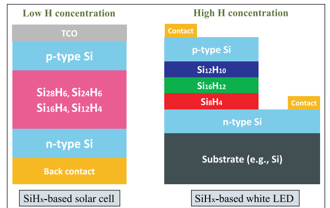
FIG. 10. Summary figure. Unusual optoelectronic properties of hydrogenated bilayer silicon: From solar absorber (low H concentration) to light-emitting diode (high H concentration) applications.
