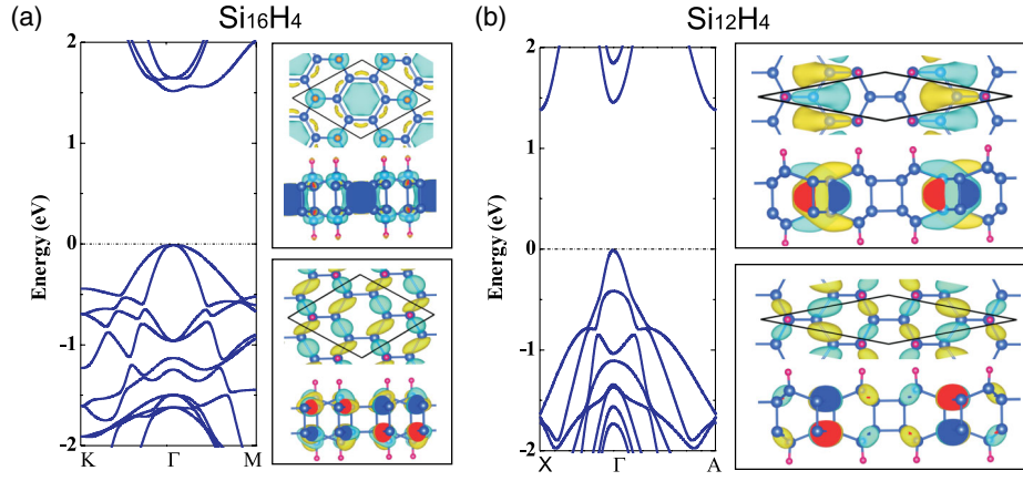
FIG. 7. The calculated band structures of double-sided (a) \text{Si}_{16}\text{H}_4 and (b) \text{Si}_{12}\text{H}_4 . The wave functions of VBM (bottom figure) and CBM (top figure) at the \Gamma point for each structure are also plotted here. The Fermi level is set to zero.
