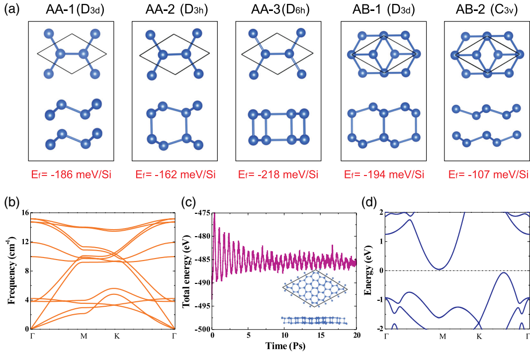
FIG. 1. (a) The structure and symmetry of five BS structures with AA or AB stacking. The formation energy E_f of each structure with respect to single-layer silicene is also plotted. (b) The phonon spectrum of the AA-3 structure. (c) The fluctuation of total energy of (100-atoms/cell) the AA-3 structure as a function of the molecular-dynamic simulation step at 600 K. (d) The calculated band structure of the AA-3 structure.
