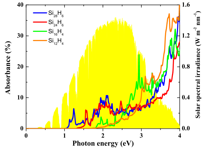
FIG. 8. The calculated optical absorbance spectra of \text{Si}_{28}\text{H}_6 , \text{Si}_{24}\text{H}_6 , \text{Si}_{16}\text{H}_4 , and \text{Si}_{12}\text{H}_4 . The reference air-mass 1.5-solar-spectral irradiance is plotted in yellow.
