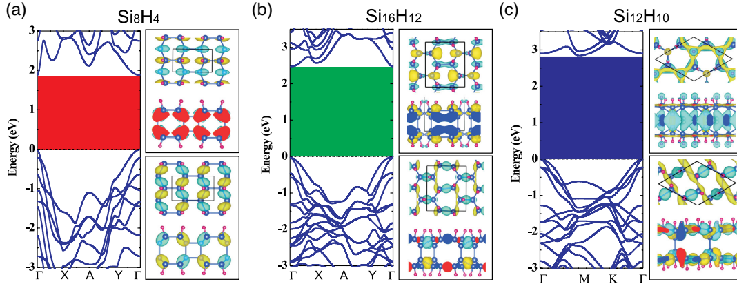
FIG. 9. The calculated band structures of double-sided (a) \text{Si}_8\text{H}_4 , (b) \text{Si}_{16}\text{H}_{12} , and (c) \text{Si}_{12}\text{H}_{10} . The wave functions of VBM (bottom figure) and CBM (top figure) at the \Gamma point for each structure are also plotted here. The color for each band gap is also shown. The Fermi level is set to zero.
