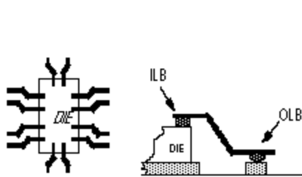
Figure 3. TAB Component
