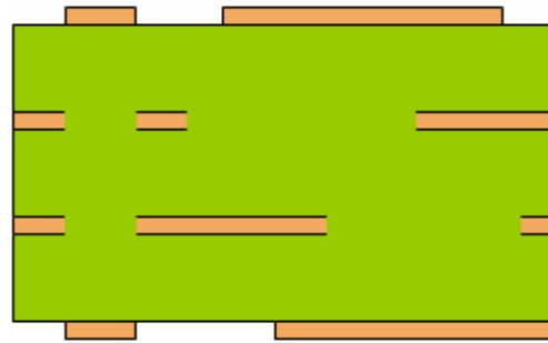
Figure 5 Etch laminated 2P core
