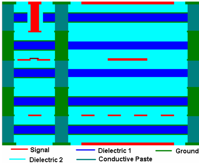
Figure 12 Mixed dielectric stack-up
