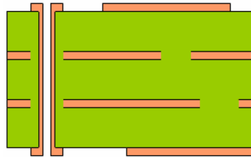
Figure 6 Drill and plate laminated 2P core
