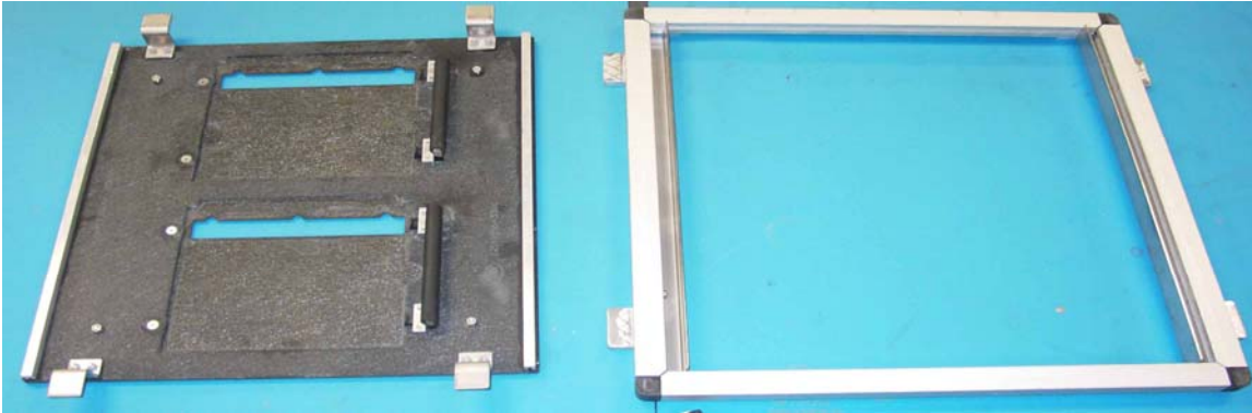
Photo 1 Wave solder pallet and insert
