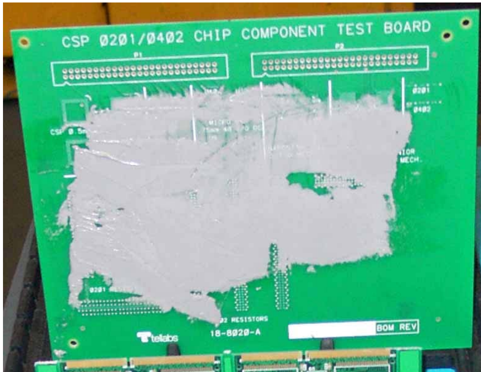
Photo 5 Test panel with solder paste applied
