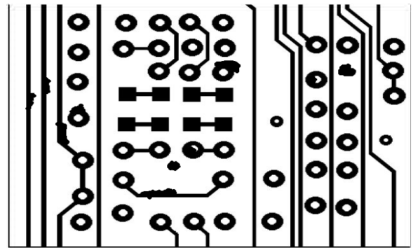
Fig12. Under etching
