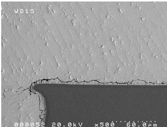
Figure 46: Board Side Failure of BGA with SAC305 Solder on ENEPIG Finish, 170 T g Board
