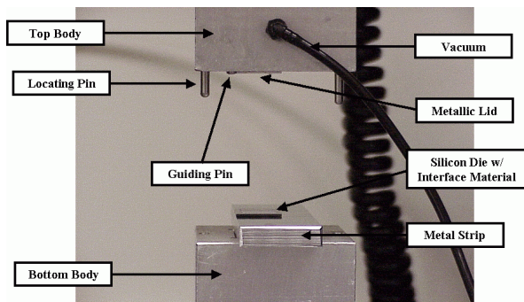
Fig.6 Placement Fixture
