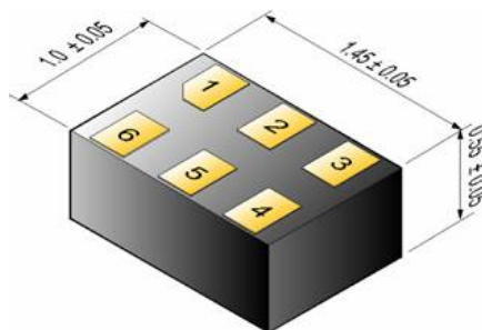
Figure 2: SMT RFID device
