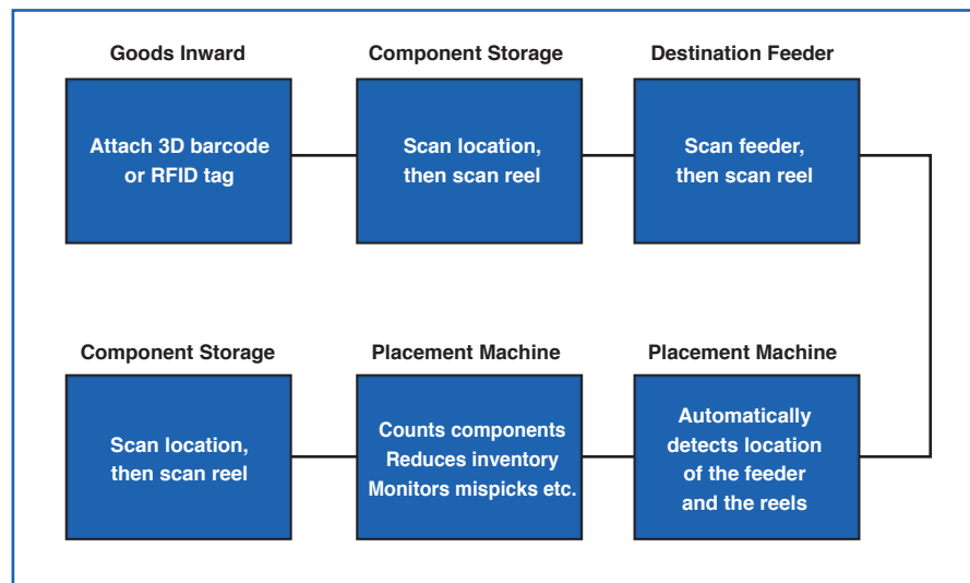
Figure 3. Flowchart showing the information flow from goods inward to post-placement.
