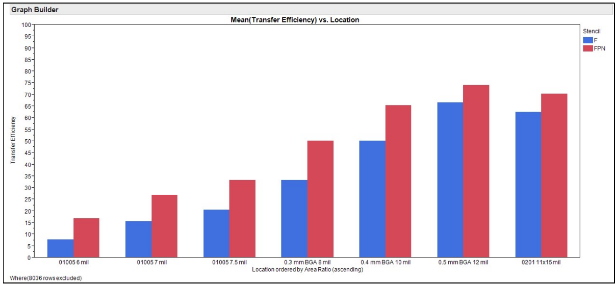
Figure 5 – Mean TE% by Location for 4 mil Thick Stencils (F-blue, FPN-red)
