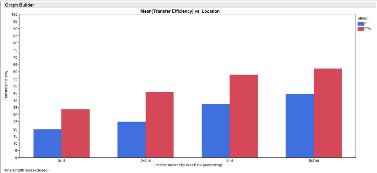
Figure 15 – 03015 Metric Stencils Mean TE% by Aperture Size, 3 mil Thick Uncoated (F) (Blue) and Nano-coated (FPN) (Red) Stencils, Type 5 Solder Paste
