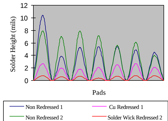
Figure 6. Height of Solder Residue Before and After Redressing (in mils)
