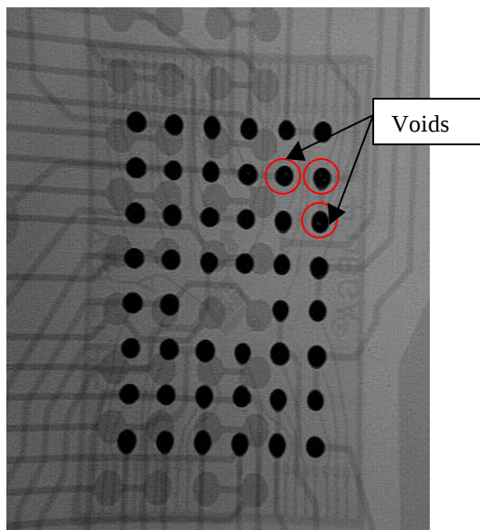
Figure 3. X-ray Image of Package B Assembly
