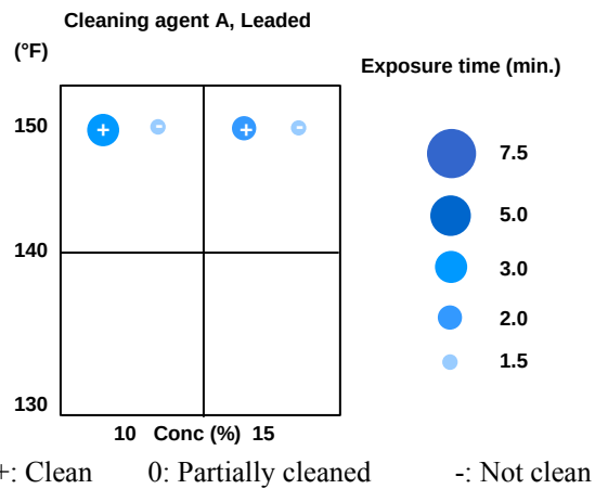
Chart 5: Cleaning agent A removing lead-free and leaded under low stand off – Phase 3
