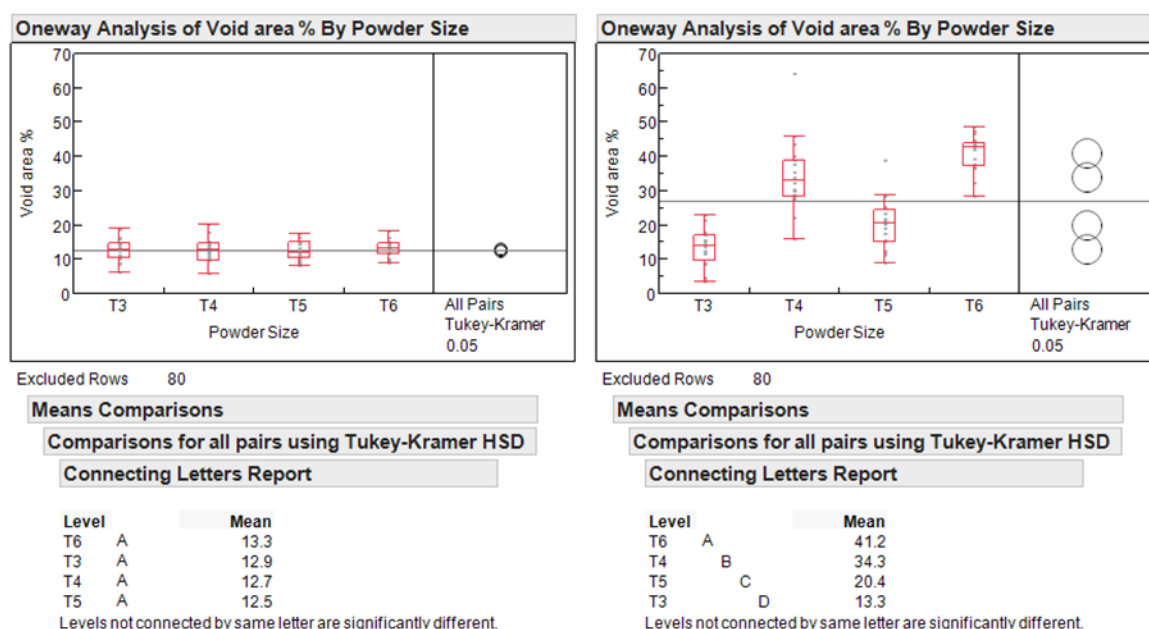
Figure 25 – Voiding for Each Solder Paste in the QFN Thermal Pads. No Clean (Left) and Water Soluble (Right)
