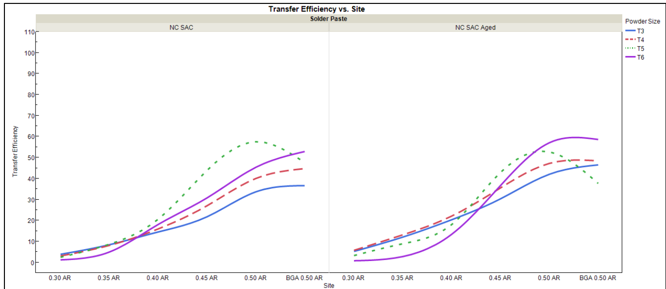
Figure 32 –Print Performance for the No Clean Solder Pastes Before and After Heat Aging
