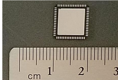
Figure 13 – QFN (MLF68) Dummy Component
