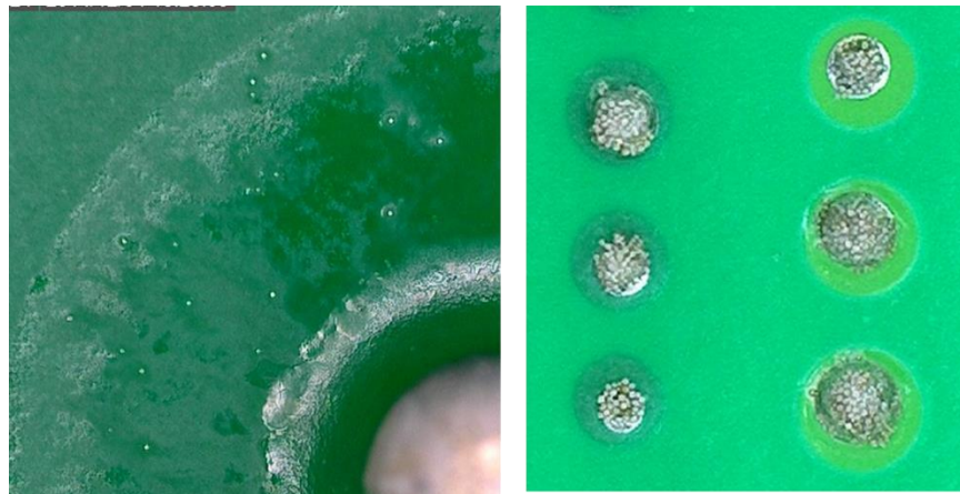
Figure 4 – Random Solder Balling (Left) and Graping (Right)
