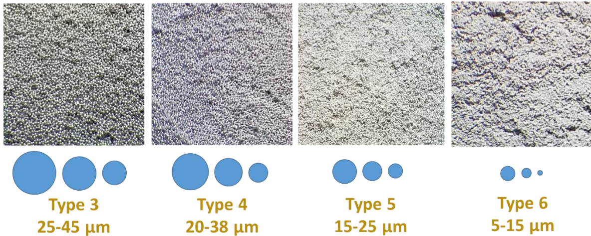
Figure 2 – IPC Type 3, 4, 5 and 6 Solder Powders
