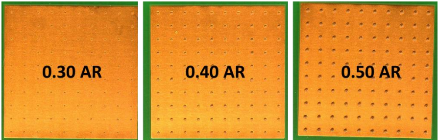
Figure 8 – Printed Solder Paste in the Area Ratio Limit Patterns
