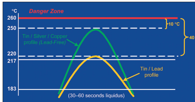
Figure 3: Lead-free process window
