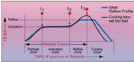
Fig.11. Accelerated rate if cooling. Decrease cooling fan speed.
