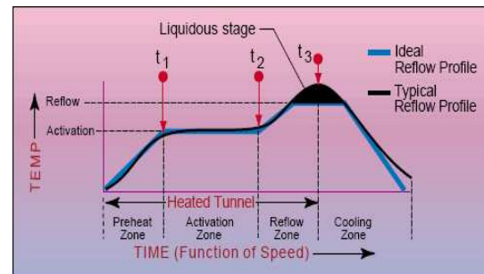
Fig.1. An example of a theoretically ideal reflow profile made up of four zones – the first three are heating and the last is cooling.
