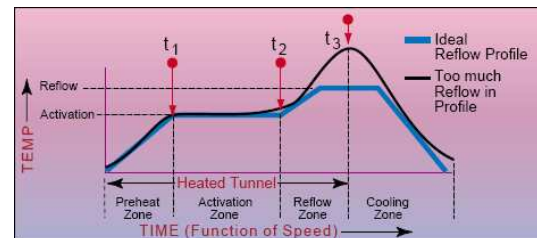
Fig.9. Reflow heat too high. Decrease temp in reflow zone.
