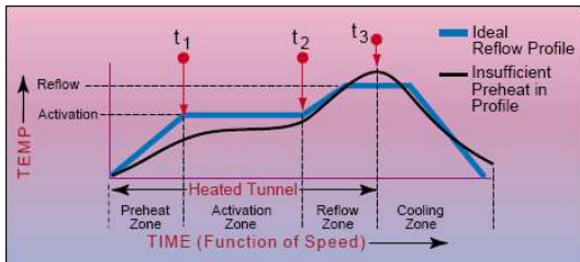
Fig.5. Insufficient preheat. Increase temp in preheat zone.
