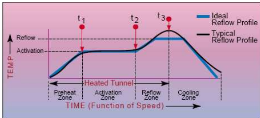
Fig.4. Profile shape for three zones plus cooling.
