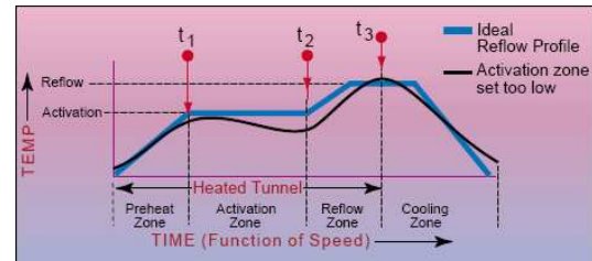
Fig.8. Insufficient activation heat. Increase temp in activation zone.
