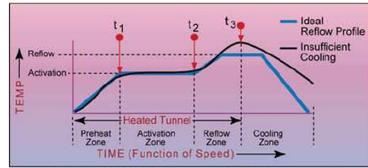
Fig.12. Insufficient rate of cooling. Increase the speed.
