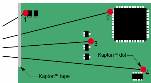
Fig.2. Fasten wires on trailing end of board with Kapton tape or dots to keep thermocouple wires from tangling on board.
