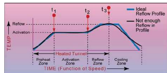
Fig.10. Insufficient heat in reflow. Increase temp in reflow zone.
