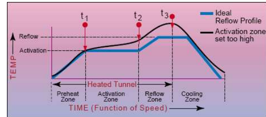
Fig.7. Activation heat too high, Decrease temp in activation zone.
