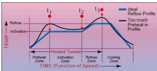
Fig.6. Too much preheat, decrease temp in preheat zone. increments. Once experience is gained with a particular oven, a better “feel”
