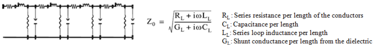
Figure 2 - RLGC model for an ideal lossy transmission line
