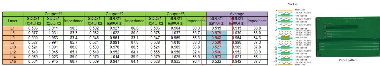
Figure 4 – 16L stackup, circuit pattern and measuring data
