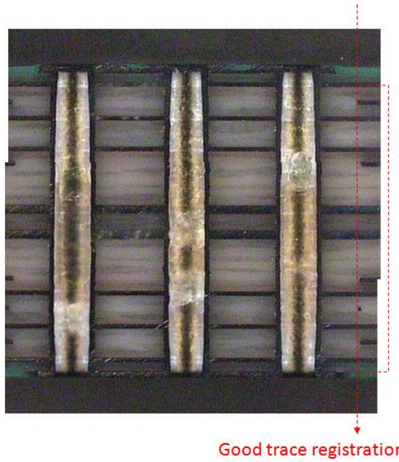
Figure 6 – Layer registration
