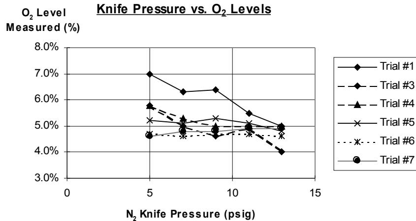
Figure 3. Nitrogen Knife Oxygen Entrainment
