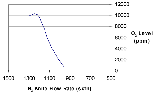
Figure 4. Oxygen Control in Econopak Plus With Hot Knife
