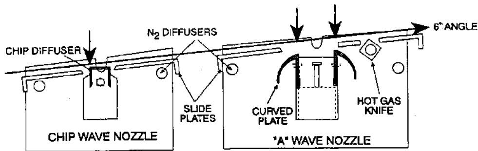
Figure 1. Wave Solder Layout [7]
