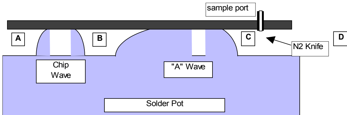
Figure 2. Wave Solder Components in Test Setup
