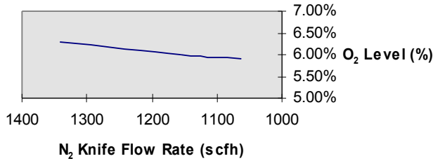
Figure 5. Oxygen Entrainment at Laminar Wave
