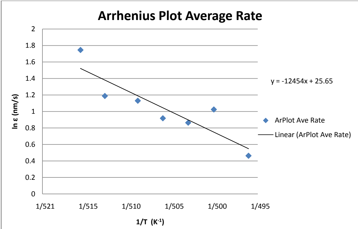
Figure 3 The Arrhenius plot was derived using data in Table 2. The equation to the right follows slope-intercept form. The slope ( m ) would be activation energy over the negative gas constant \left(-\frac{Q}{R}\right) and the y-intercept ( b ) would be the frequency factor ( \ln A ).
