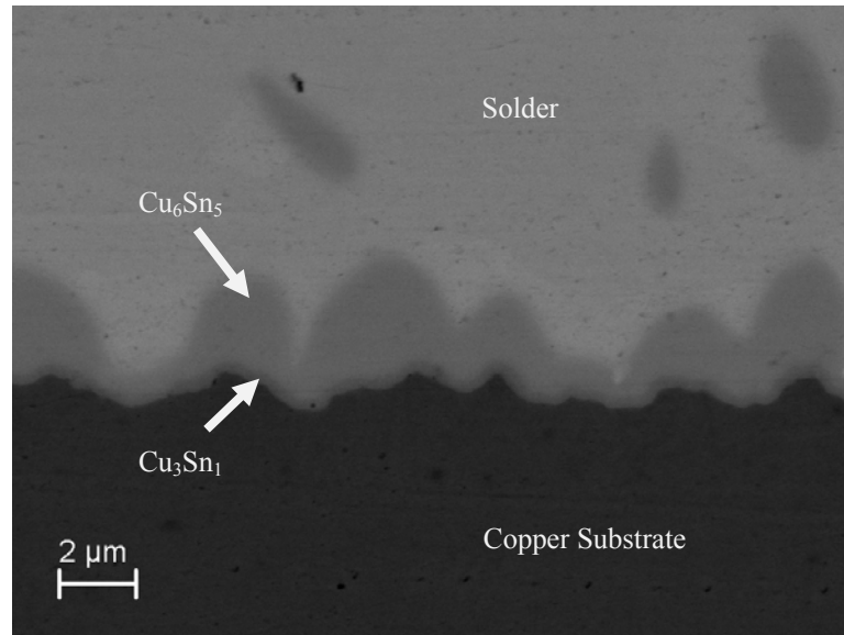
Figure 2 First and second layer intermetallics are present in this sample that was manufactured at a reflow temperature of 223^\circ\text{C} and held above liquidus for 105 seconds.
