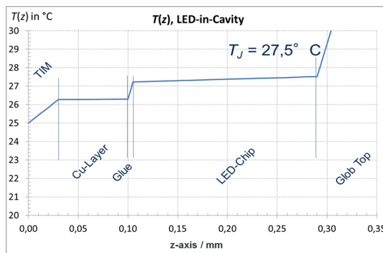
Figure 13. Results: Temperature profile along the symmetry axis in out-of-plane direction ( z -axis) of a LED-in-Cavity set-up
