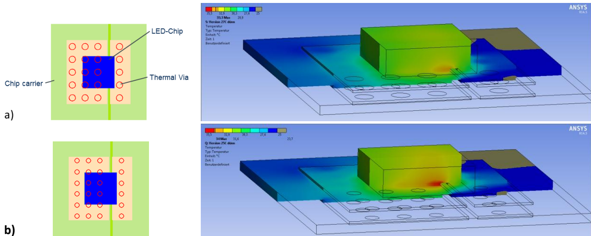
Figure 17. Chip carrier design and first results of thermal simulation: a) 20 vias, d = 200 \mu\text{m} ; b) 24 vias, d = 150 \mu\text{m}
