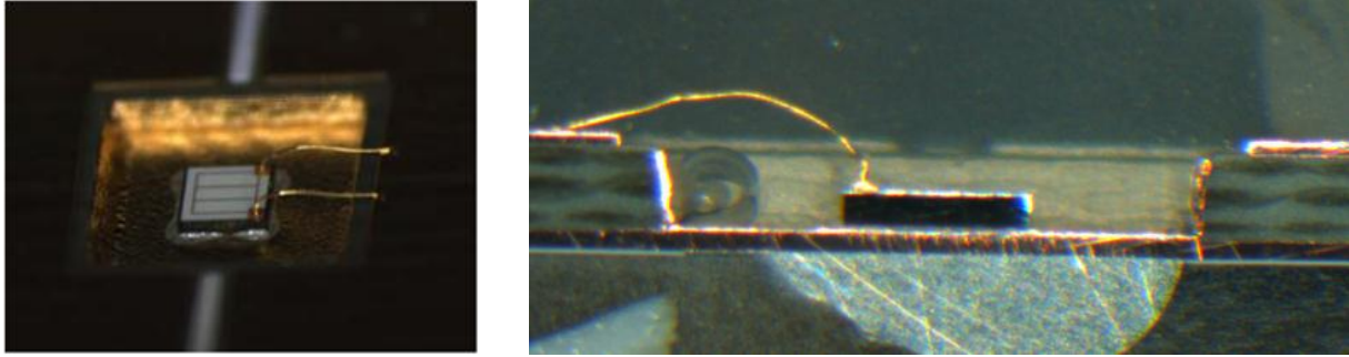
Figure 8. Chip in cavity bonded to the upper layer
