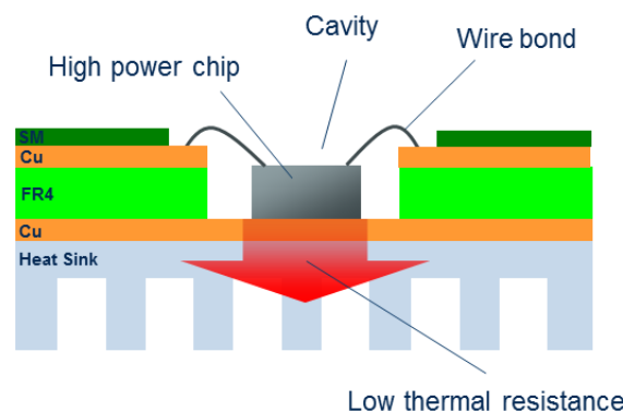
Figure 7. Chip in cavity build-up with optimized thermal path
