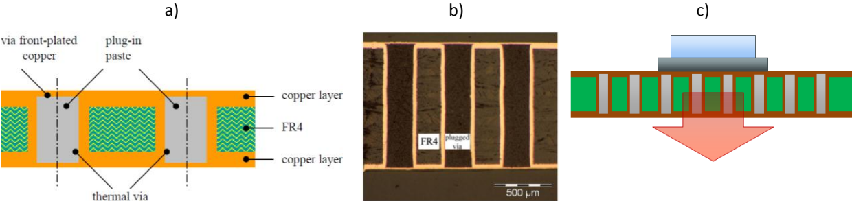
Figure 3. PCB with plugged thermal vias: a) Scheme; b) cross section; c) thermal path
