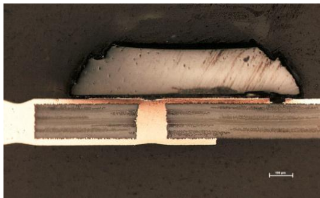
Figure 18. Chip carrier with dimple inside via
