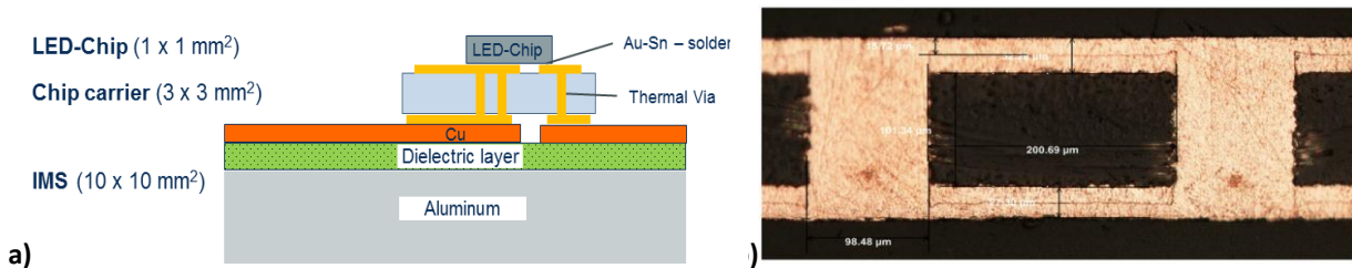
Figure 16. a) Chip carrier module build-up; b) cross section of chip carrier
