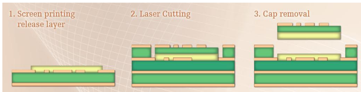
Figure 6. Schematic process flow of cavity formation
