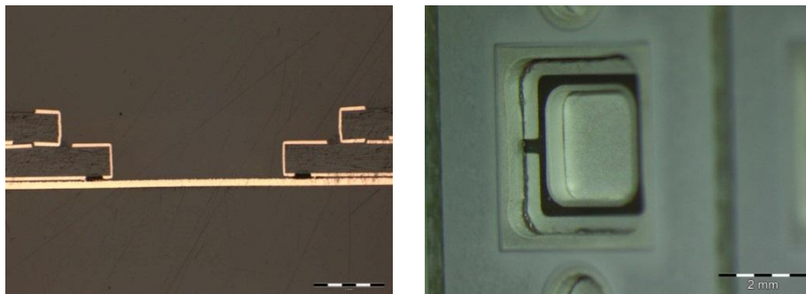
Figure 9. Cavity in cavity board with high reflective cavity walls
