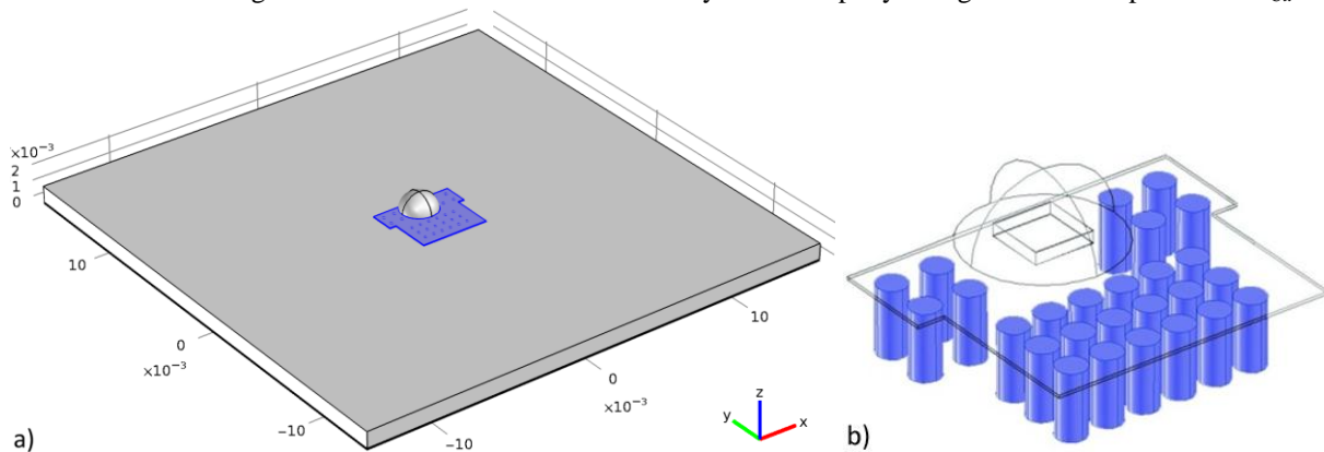
Figure 11. Thermal model of the FR4-DK test sample: a) Entire model; b) detailed view thermal via array
