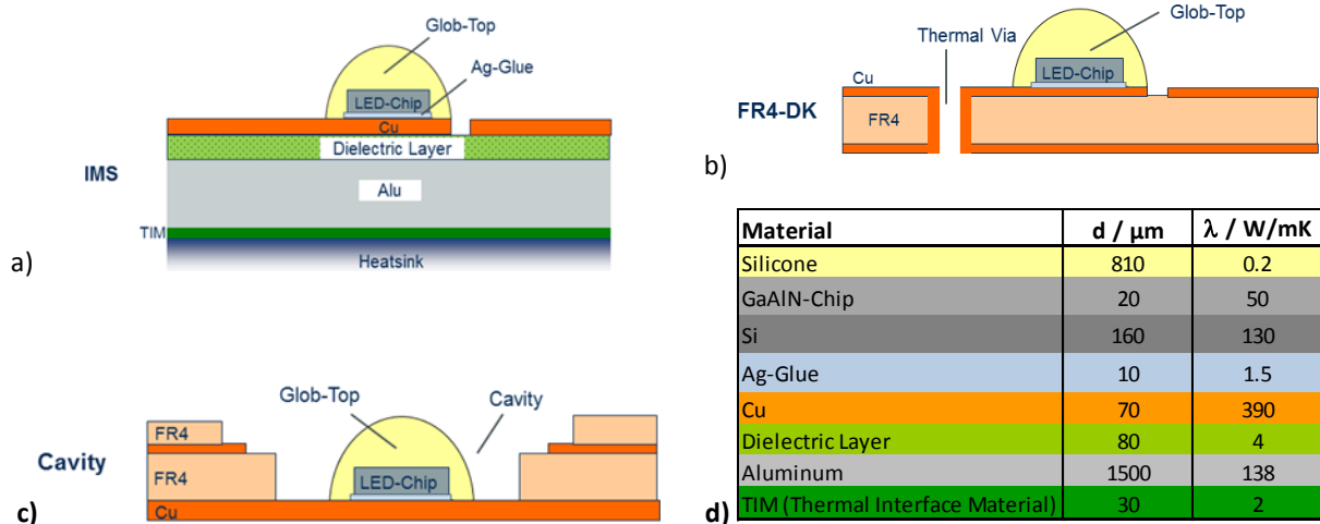
Figure 10. Build-up of: a) IMS, b) FR4-DK, and c) Cavity board (LED-in-Cavity); d) material parameters used for thermal simulation
