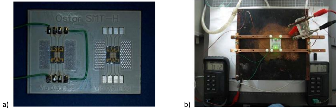
Figure 4. LED module mounted on water-cooled heat sink: a) Top view of test sample; b) sample under test
