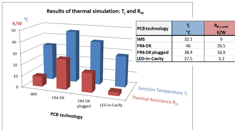
Figure 15. Comparison of the results of the different PCB technologies
