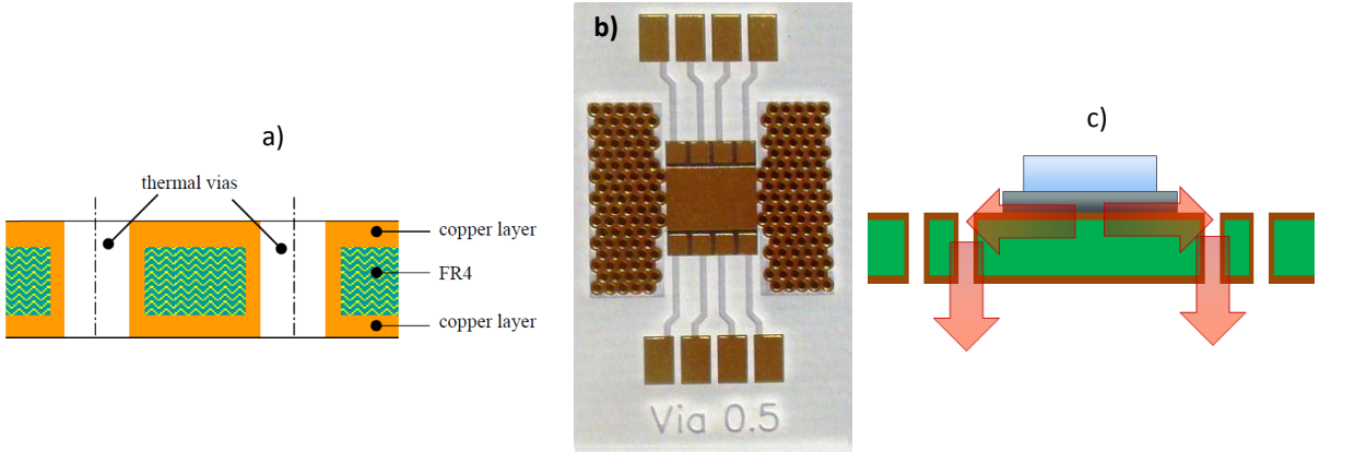
Figure 2. PCB with open thermal vias: a) Scheme; b) design; c) thermal path
