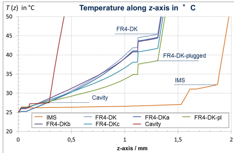
Figure 14. Comparison of the results of the different PCB technologies
