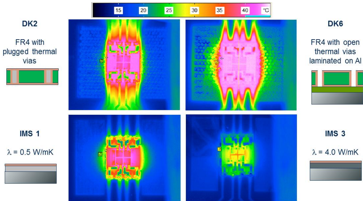
Figure 5. Comparison of results obtained from IR thermography measurements
