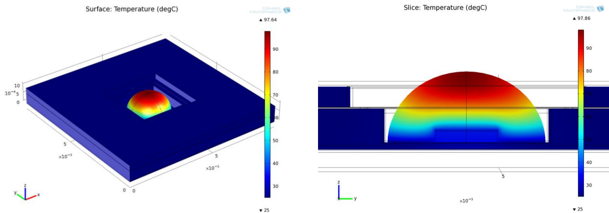
Figure 12. Results of thermal simulations; detailed views of temperature distribution in vicinity of the LED
