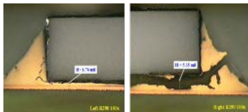
SnCuNi
