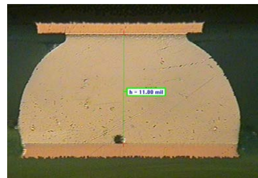
Material C
