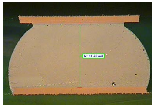
Material D
