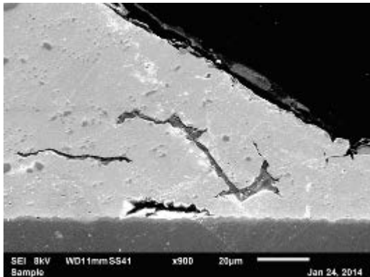
SAC305: ductile fracture propagating along intermetallic grain boundaries
