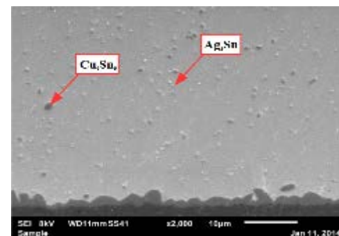
Material C
