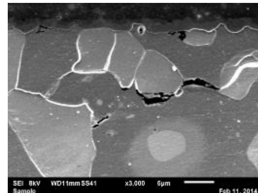
SnBiAg: grain boundary sliding between Sn and Bi dendrites
