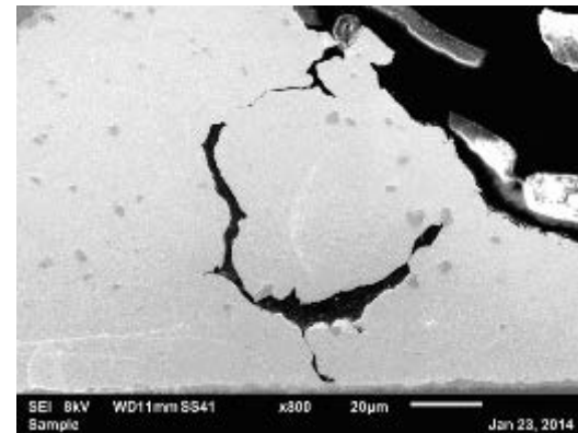
SAC0307, SnCuNi, Alloy C: ductile fracture along Sn grain boundaries
