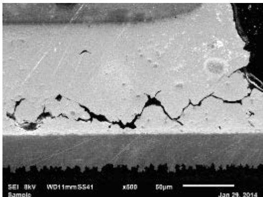
Alloy D: ductile fracture along Sn grain boundaries
