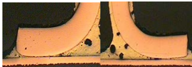
SnCuNi
