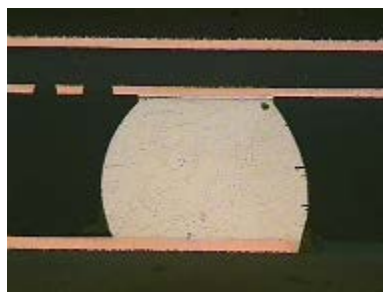
SnCuNi
