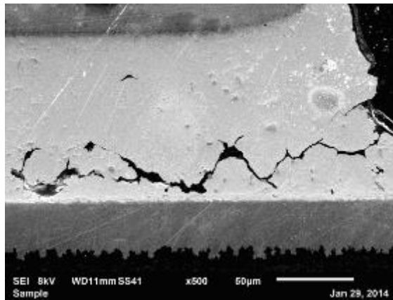
Figure 24. Cracking along Sn grain boundaries in QFN88 solder joint assembled using Material D
