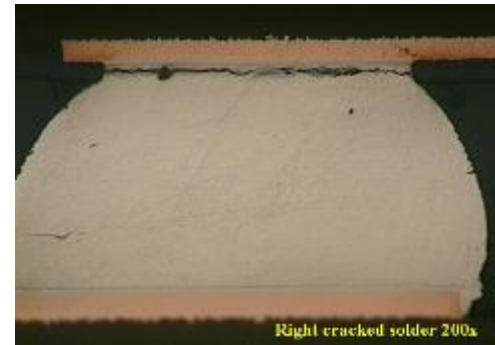
Material C
