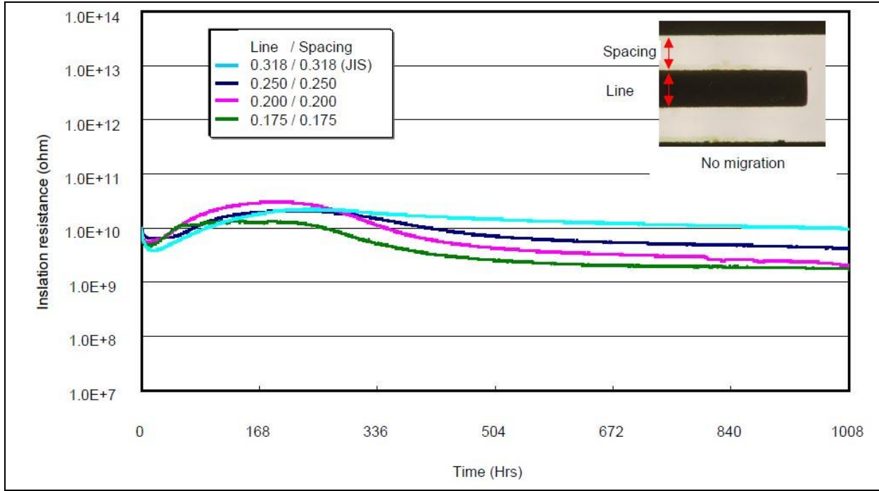
Figure 14: Crack-free reflowed Paste A conventional high temperature/humidity SIR testing data with 0.318mm, 0.25mm, 0.2mm, 0.175mm line widths and spacings.
