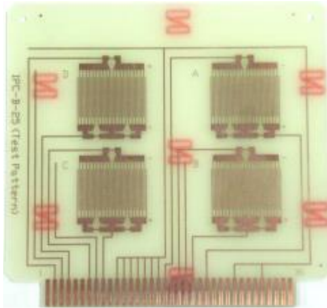
Figure 3: IPC-B-25 test board (E pattern)
