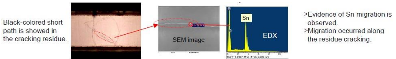
Figure 11: Conventional Reflowed Paste B after Dew test method (A) testing
