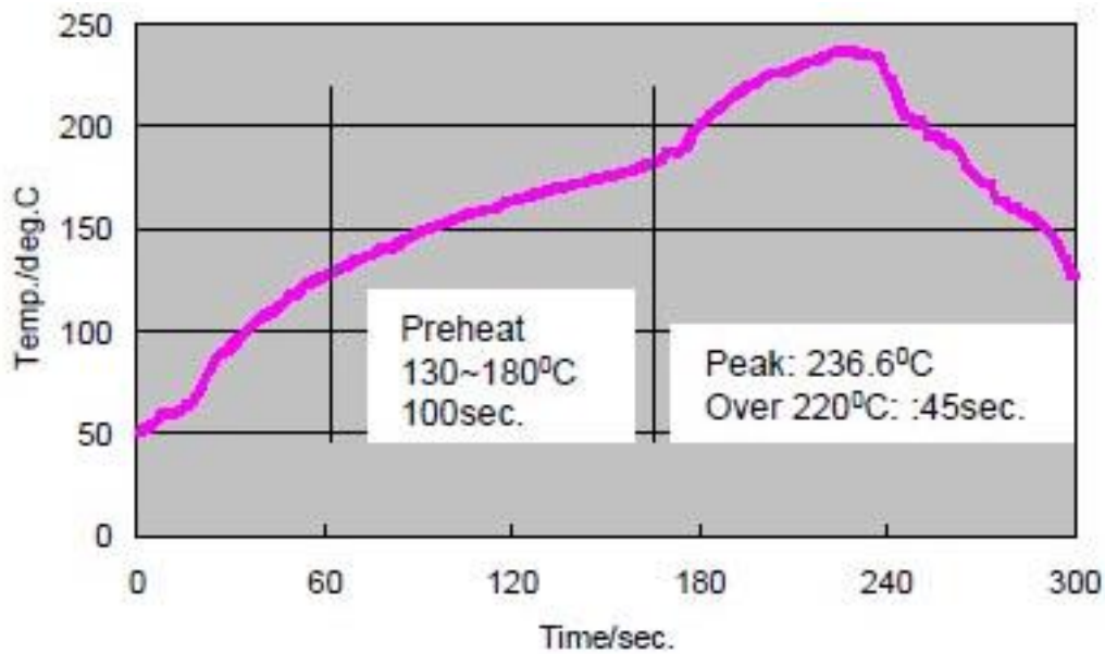
Figure 2: Lead-free reflow profile used
