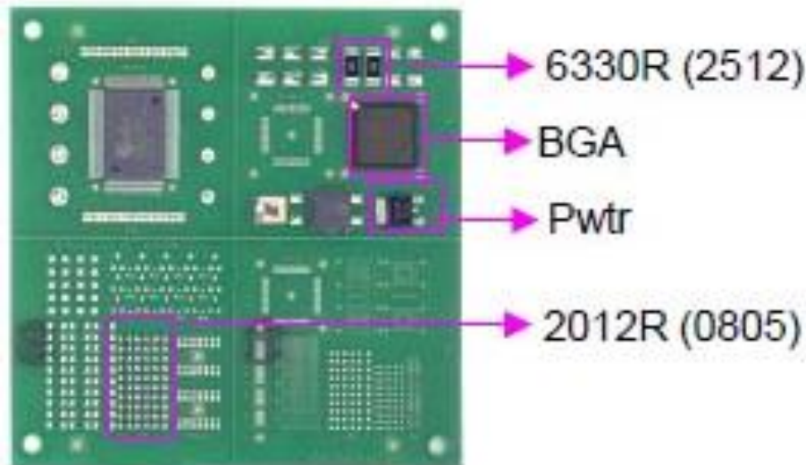
Figure 8: Company Test Board for Voiding/Reflow Testing
