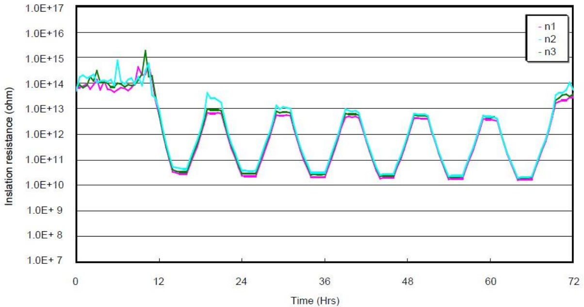
Figure 13: Crack-free reflowed Paste A during Dew test method (B) testing
