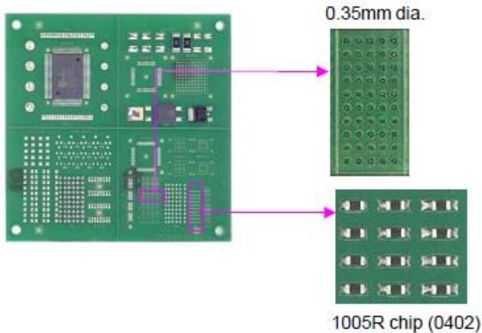
Figure 7: Company Test Board for Wetting/Reflow Testing
