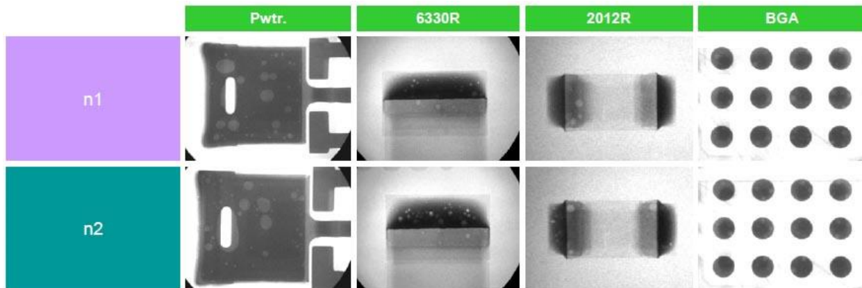
Figure 19: Crack-free Paste A reflow/voiding test data for soldered Power transistor, 6330R chip, 2012R chip and BGA components.
