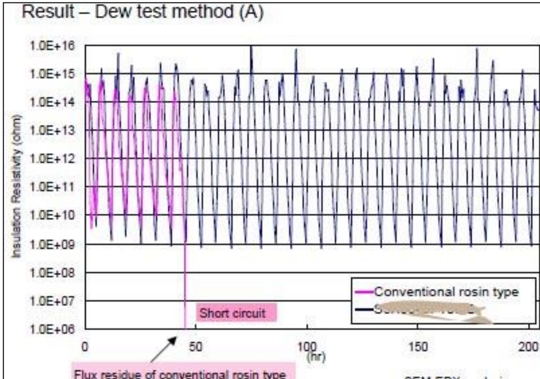
Figure 10: Crack-free reflowed Paste A versus conventional reflowed Paste B during Dew Test method (A) testing
