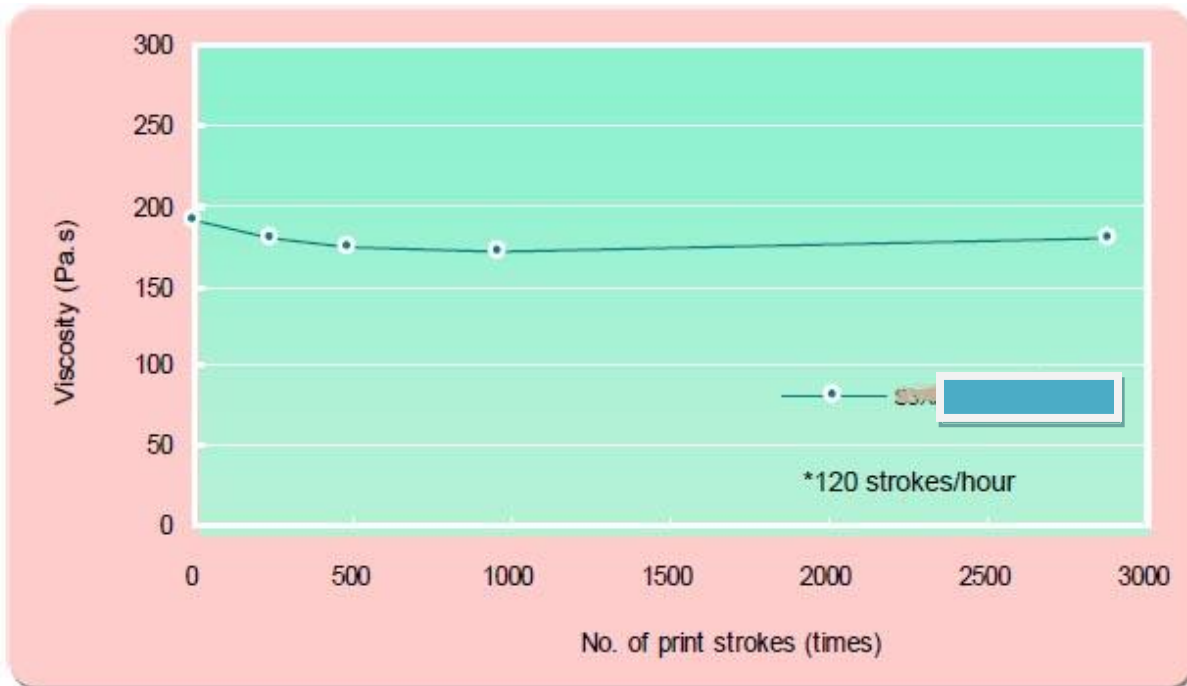
Figure 17: Crack-free Paste A viscosity data over a 24-hour paste printing period
