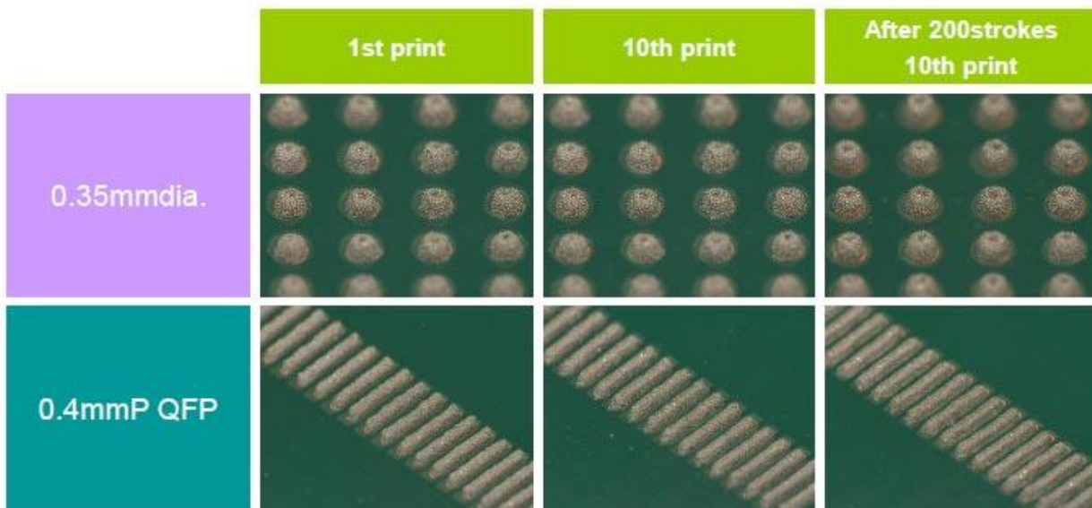
Figure 15: Crack-free Paste A printing results on 0.35mm diameter pads and 0.4mm pitch QFP component pads.
