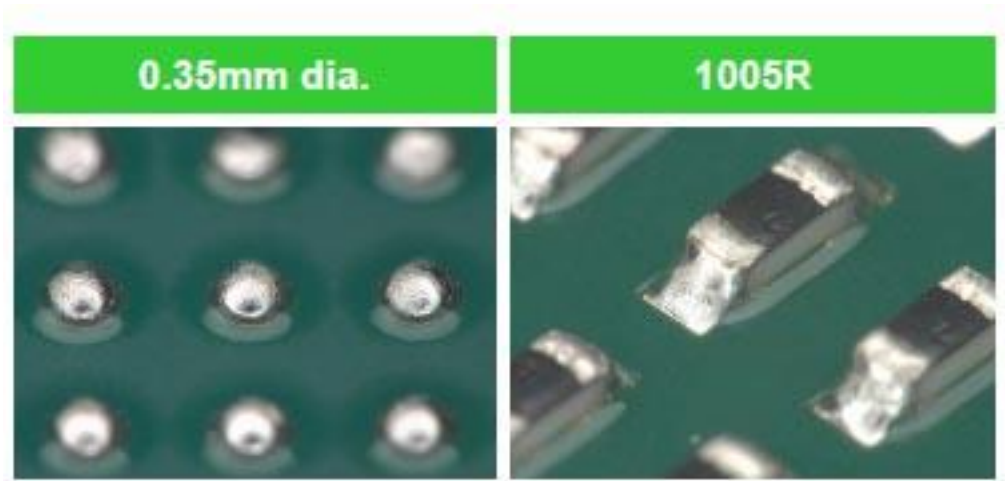
Figure 18: Crack-free Paste A wetting/reflow test data for 0.35mm diameter board pads and soldered 1005R soldered chip components.
