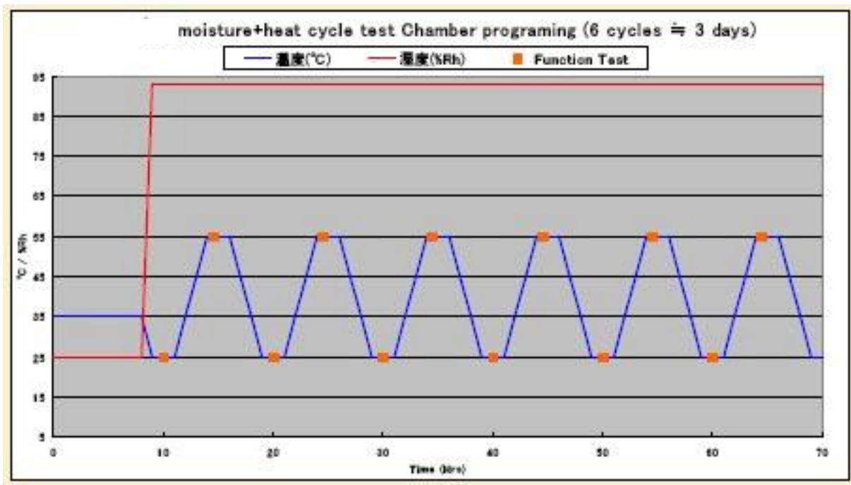
Figure 5: Dew Test Method (B) Temperature and Humidity Profile.
