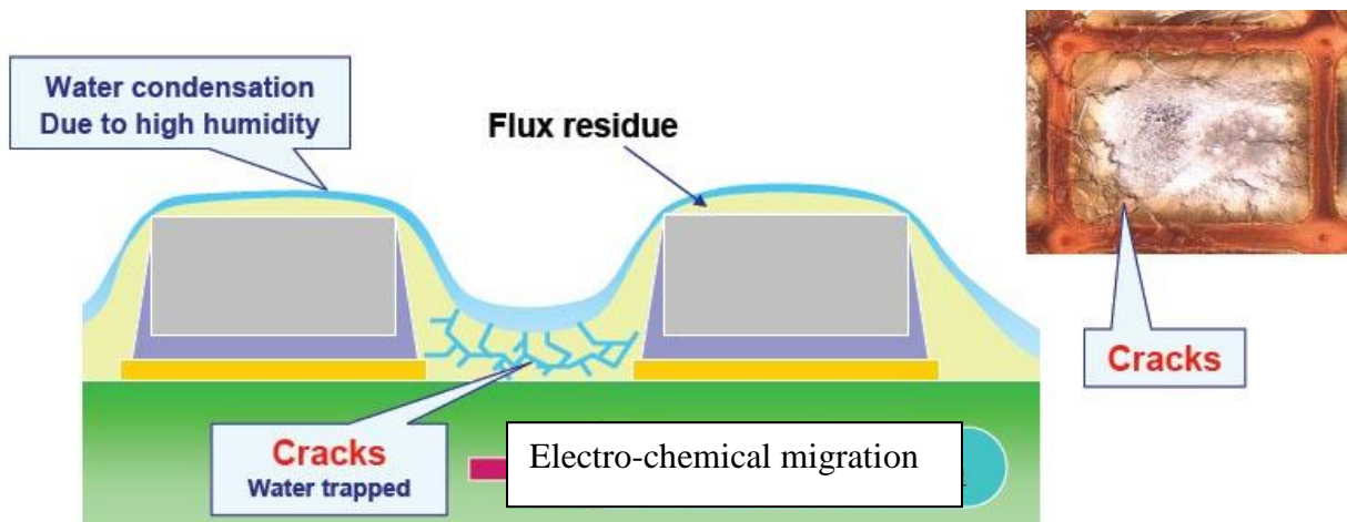
Figure 1: Effect of Flux Cracking on Reliability under High Humidity Conditions
