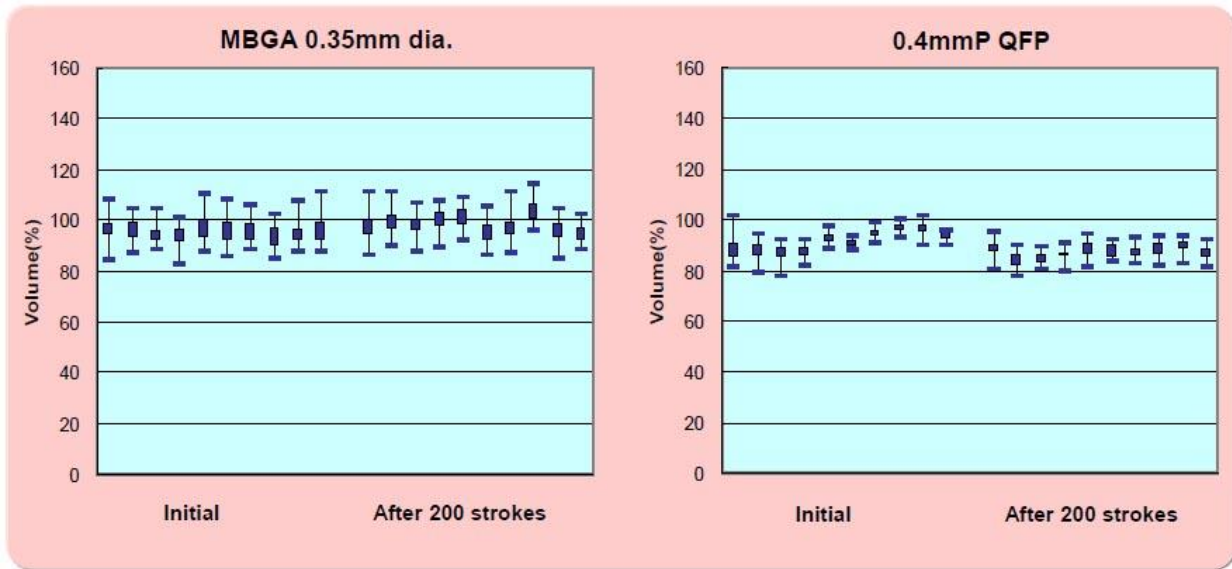
Figure 16: Crack-free Paste A printing SPI data for 0.35mm diameter BGA pads and 0.4mm pitch QFP pads.
