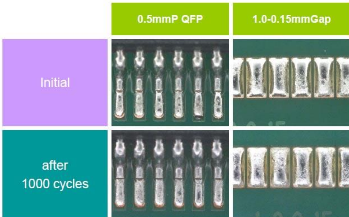
Figure 9: Cracking test on reflowed crack-free Paste A before and after thermal cycling on soldered 0.5mm pitch QFP component and 1mm wide pads with 0.15mm gaps.
