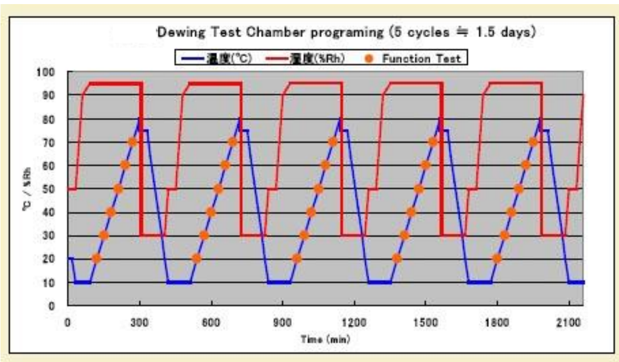
Figure 4: Dew Test Method (A) Temperature and Humidity Profile
