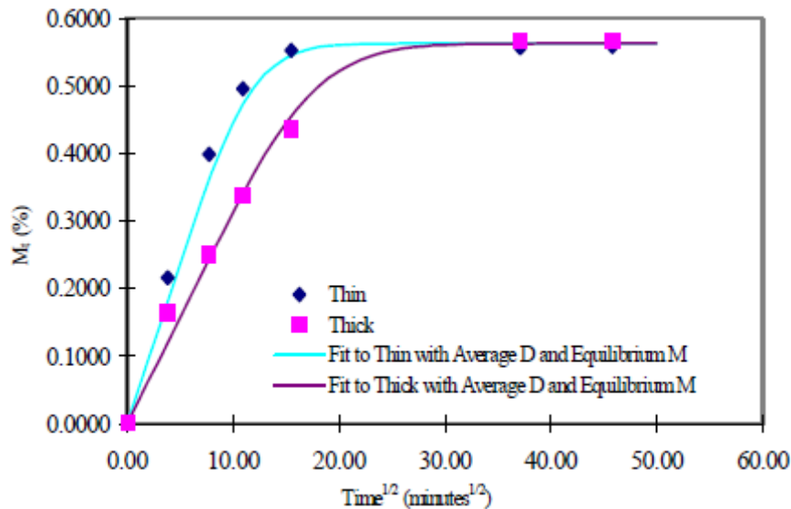
Figure 3: Diffusion curves with theoretical fit (CE-A laminates at 50 oC/85%RH).
